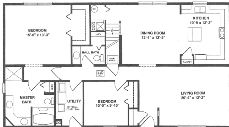
HARTFORD 28x52 (2) BEDROOM
