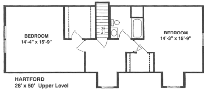
SUGGESTED UPPER LEVEL LAYOUT (Finished By Builder) Optional Dormers shown
