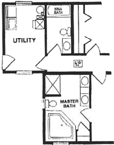
Crawspace Floor Plan
