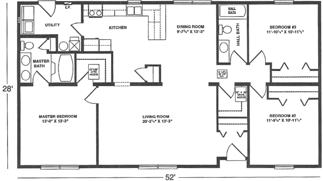
FLOOR PLAN MODIFICATIONS WITH BASEMENT OPTION
