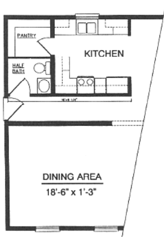
OPTIONAL JEFFERSON II Bath / Utility Layout
